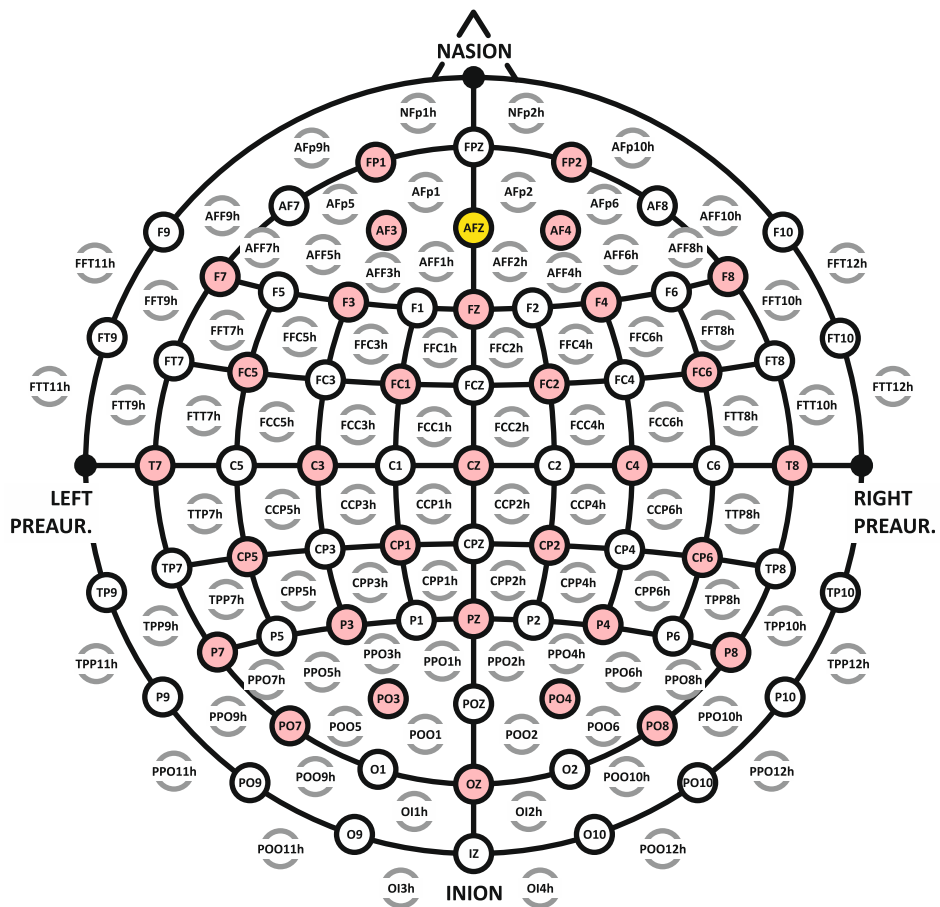
32-channel setup standard
